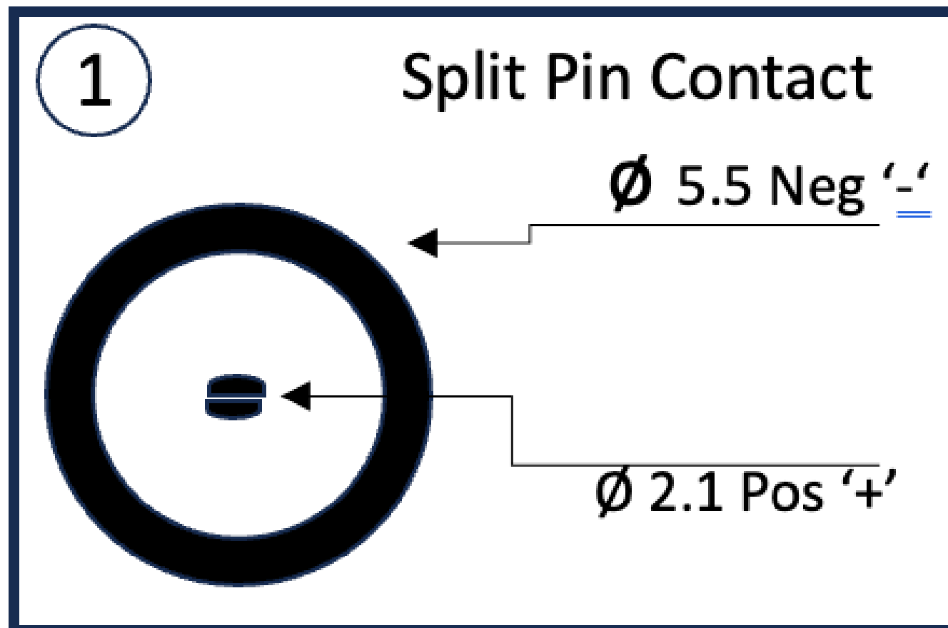
Connector A
