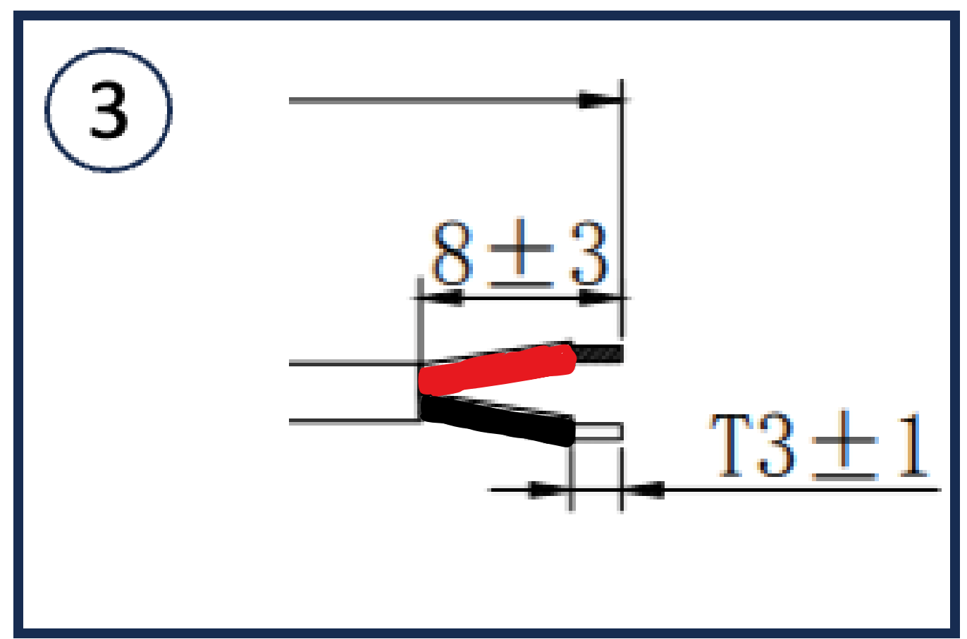
Connector B
