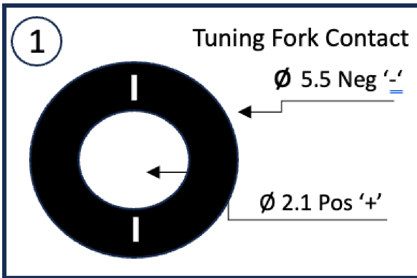
Connector A
